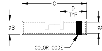
2) METAL CRIMP SPLICE
